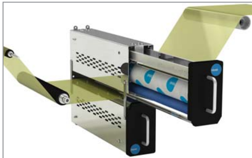
Small machines (SL & MWC) used on pilot lines or for line validation
